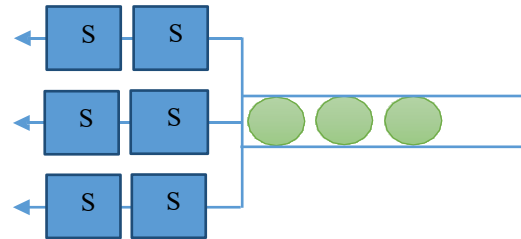
Fig. 4. Single queue, several service and multiple stages [9]
