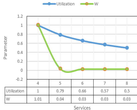
Fig. 5. Comparison between service providers
