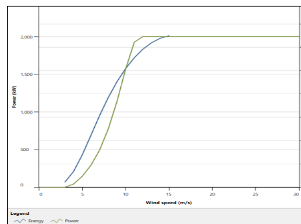
Fig 2. The relationship between wind speed, Energy and Power.
